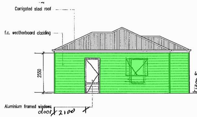
SOUTH SIDE ELEVATION SCALE 1:100
