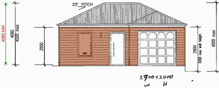
EASTERN FRONT ELEVATION SCALE 1:100
